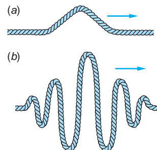
FIGURE 5-14 (a) Wave pulse moving along a string. A pulse has a beginning and an end; that is, it is localized, unlike a pure harmonic wave, which goes on forever in space and time. (b) A wave packet formed by the superposition of harmonic waves.
